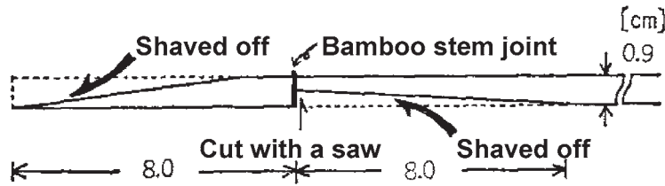
Fig. 6 Preparation of Split Bamboo
