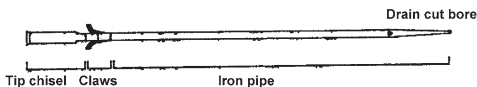
Fig. 4 Iron Pipe Schematic
