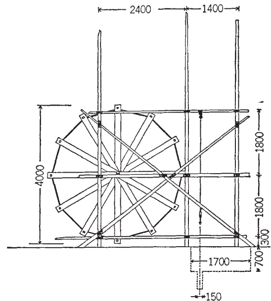
Fig. 9 Higo-guruma (bamboo wheel) on the Scaffolding
