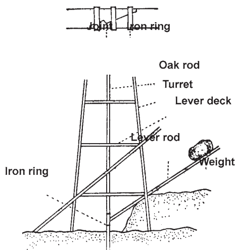
Fig. 3 Kashibo-tsuki method - Oak Rod Joints and Scaffolding (Source: Nagami's literature)
