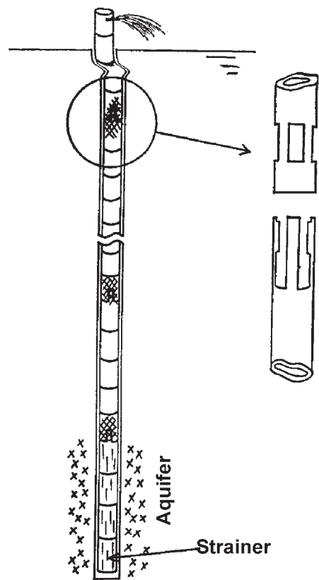
Fig. 11 Toi (vertical water duct) and its joint
